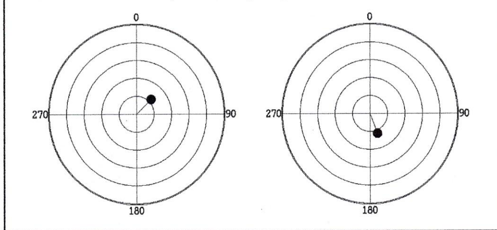
CORRECT UNBALANCE GRAPH (max = 50.0 gr )
