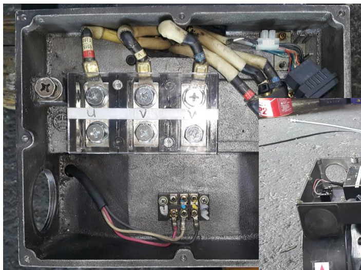
TERMINAL BLOCK 교환
