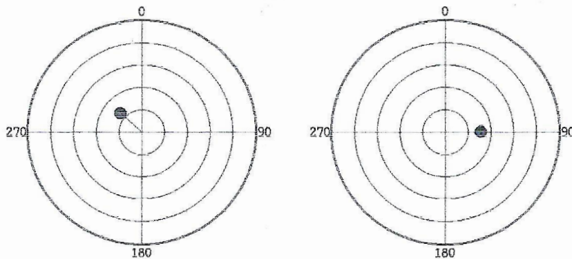
CORRECT UNBALANCE GRAPH (max = 50.0 gr )
