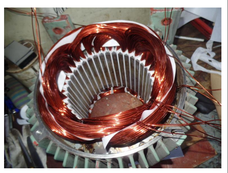
STATOR
